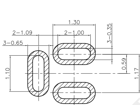
RECOMMENDED PCB LAYOUT TOLERANCE±0.05(焊盘推荐图) (FOR REFERENCE ONLY)
