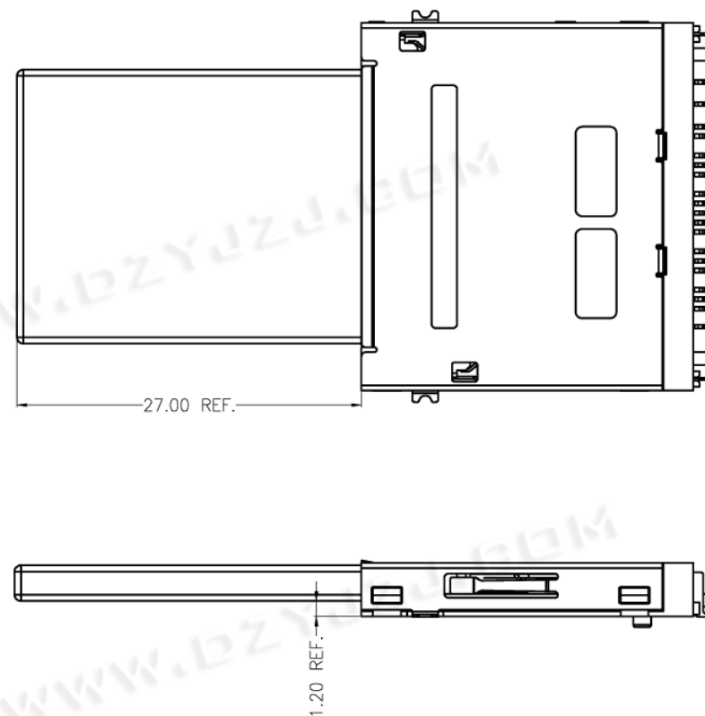
MS Card Insert Drawing:
