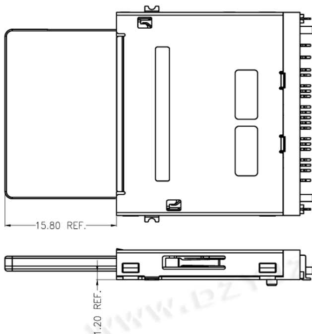
MMC Card Insert Drawing:
