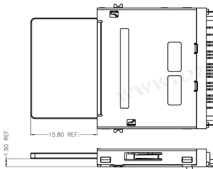
MMC Card Insert Drawing:
