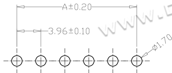
PCB LAYOUT
