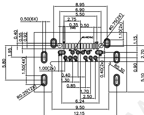
PCB LAYOUT (RECOMMENDED) (Tol: ±0.05)
