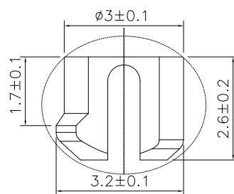
B VIEW SCALE 4/1
