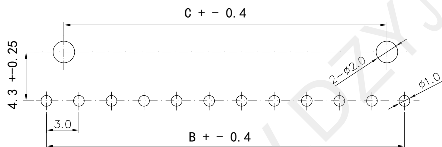
P. C. B Layout
