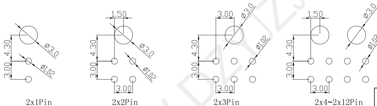
P. C. B LAYOUT
