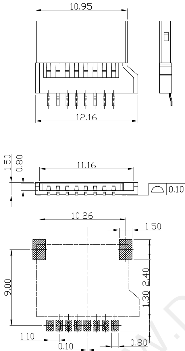
RECOMMENDED PCB LAYOUT (Witchout Post)
