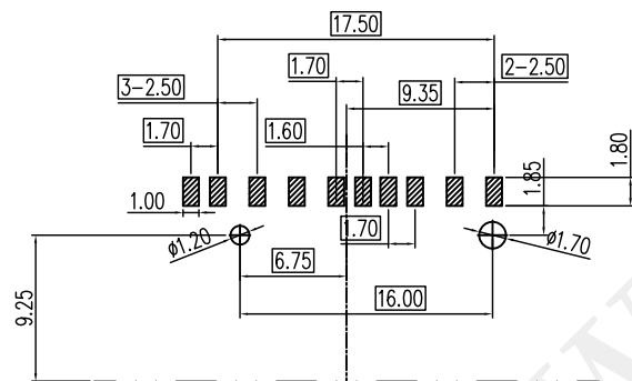
RECOMMENDED PCB LAYOUT(.XX±0.05) CONNECTOR SIDE(TOP VIEW)
