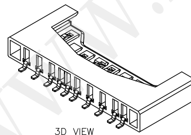
3D VIEW
