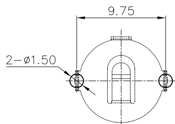
PCB Layout Diagram Bottom View
