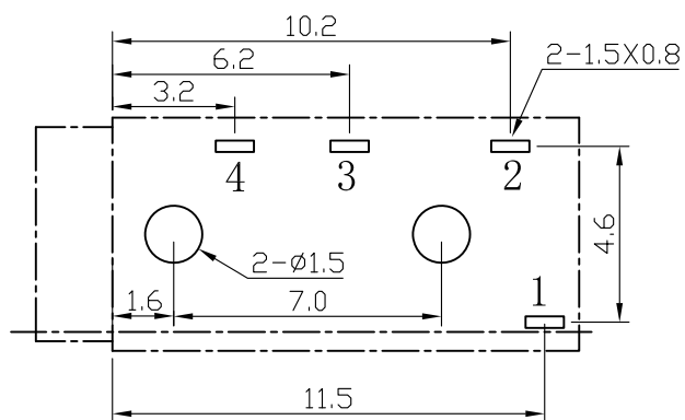
T:1.6 Dimensions of PC board holes Tolerance : \pm 0.1 (Printed-sided view)
