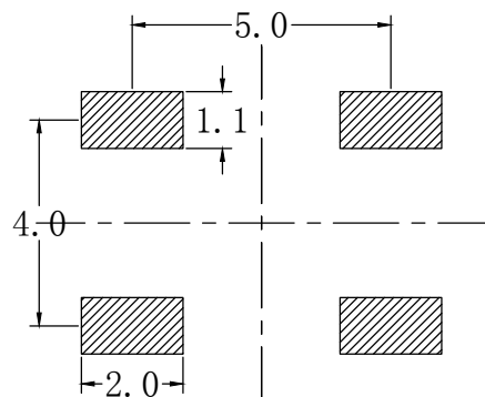
PCB.layout
