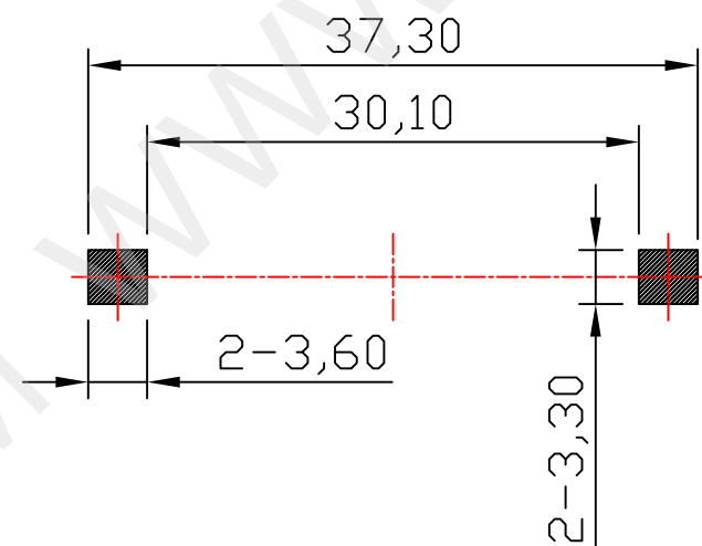
PCB Layout Diagram Top View
